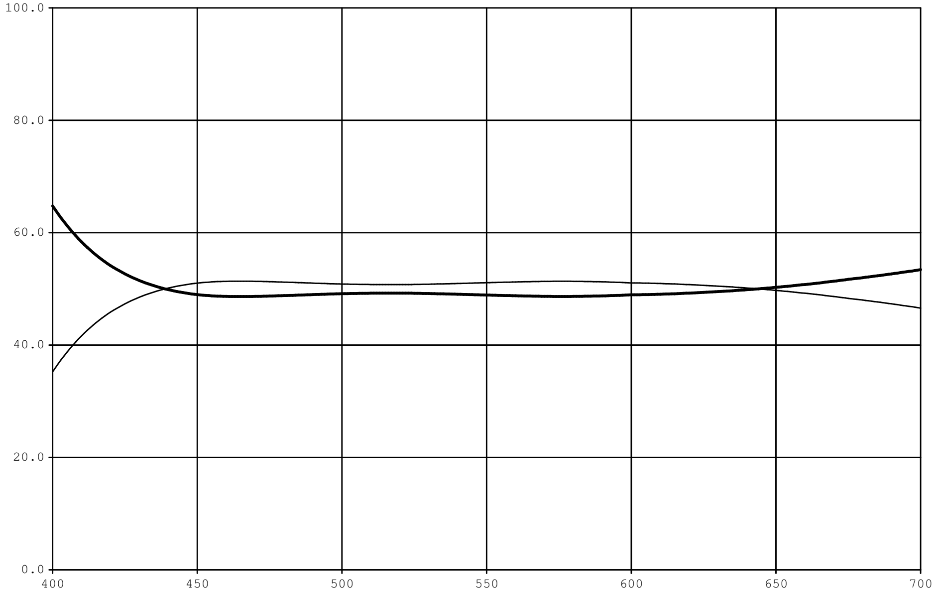
Transmittance (%) and Reflectance (%) vs Wavelength (nm)
